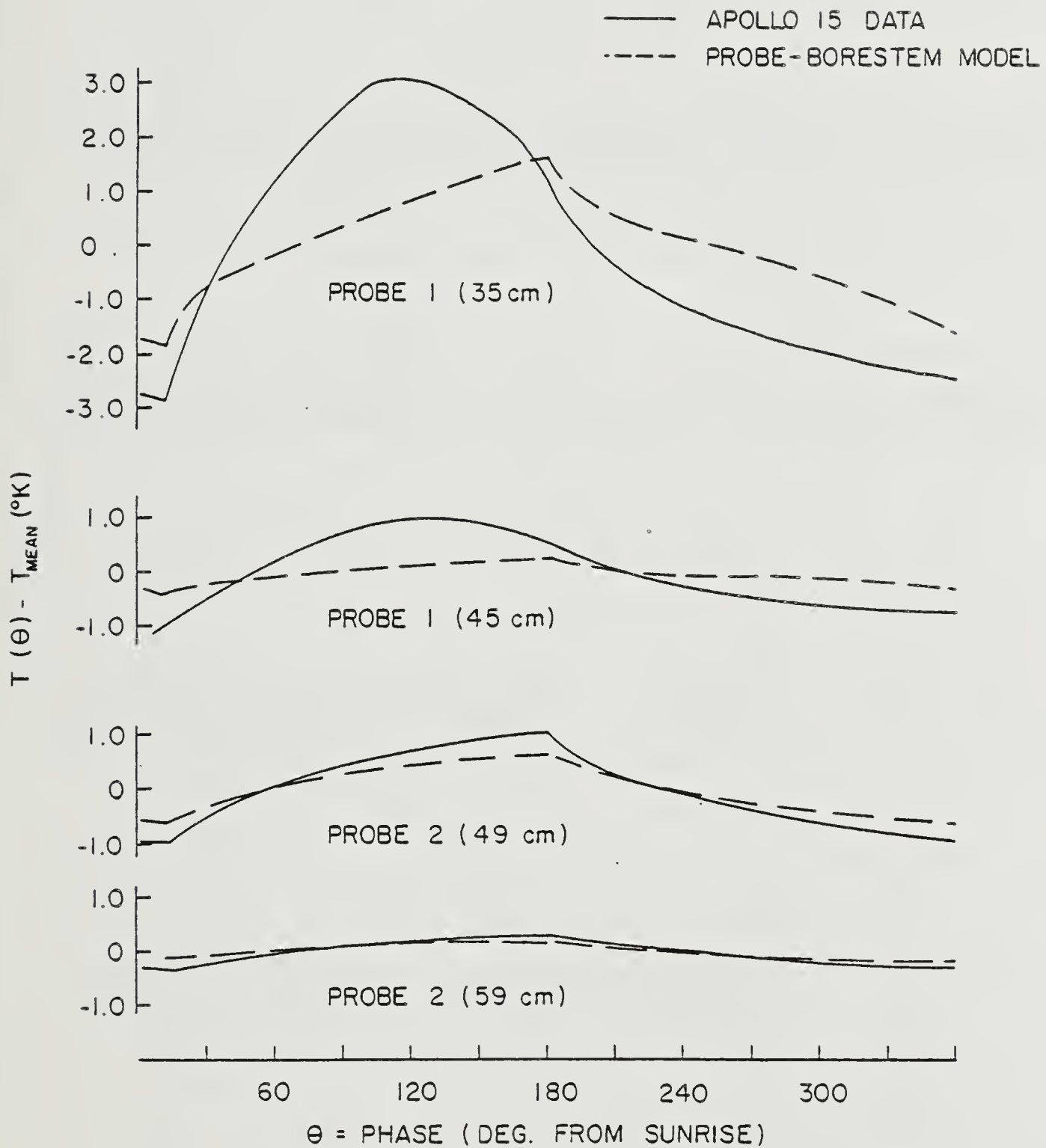
Comparison of diurnal variations observed in the Apollo 15 subsurface data and produced by the numerical models at comparable sensor depths.
